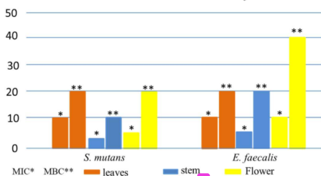
Fig.-2: MIC and MBC Value of T. procumbens against S. mutans and E. faecalis
