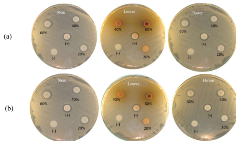
Fig-1: Activity Test Results of the Stem, Leaf, and Flower Extract of T. procumbens against bacteria (a) S. mutans , (b) E. faecalis
