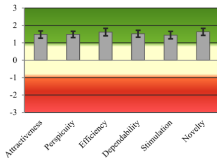
Figure 2. Graph of mean value of 6 UEQ scales
